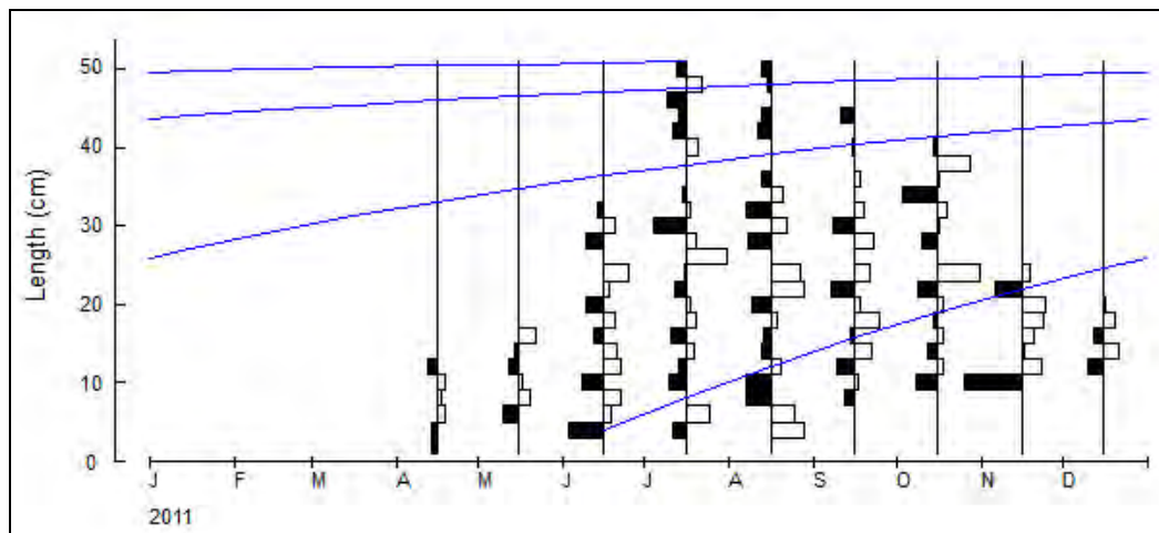
Figure 25. Growth curve superimposed over restructured length-frequency data of Pamapama .
